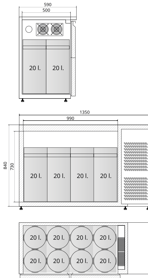
bokorys CKC8 KEG
