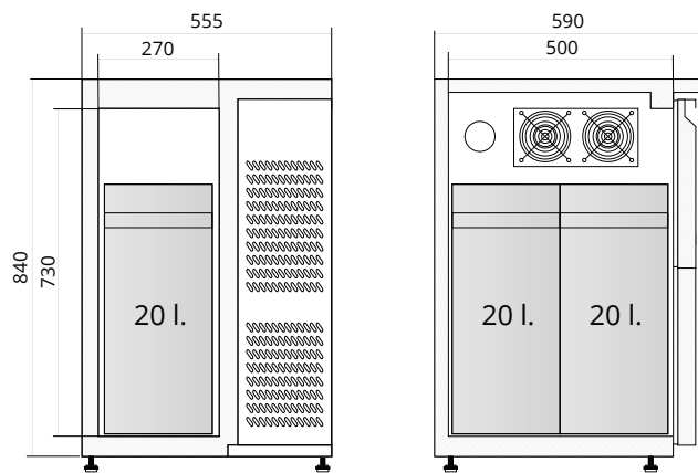
bokorys CKC2 KEG
